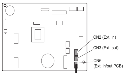
Indoor unit PCB
